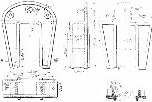
Figs. 4852-4856. PEDESTAL.
